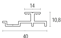
Clip in alluminio AF610
