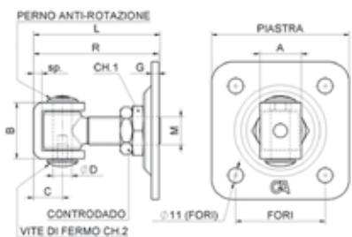
Cardine c/piastra 100x100 c/cavallotto Zincato
