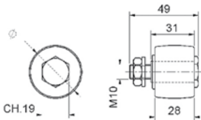
Oliva nylon bombata
