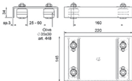
Piastra guida 4 olive bombate nylon
