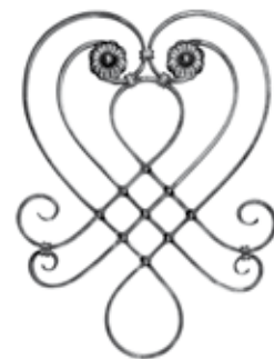
Art. L055.88.216 ■ 16x8 H mm 600 L mm 430
