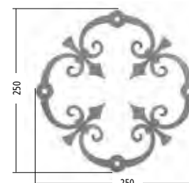
Art. D6 sp. mm 6
