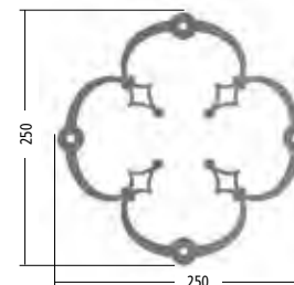
Art. D3 sp. mm 6
