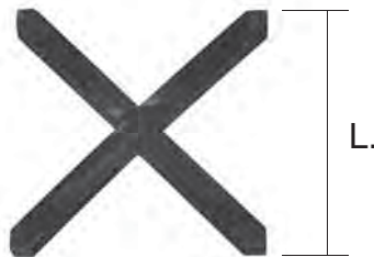
Liscio / Smooth Art. 03.034.60 \square 12 L.100 x H.100 mm Art. 03.034.61 \square 12 L.110 x H.110 mm Art. 03.034.62 \square 12 L.125 x H.125 mm Art. 03.034.63 \square 12 L.108 x H.108 mm
