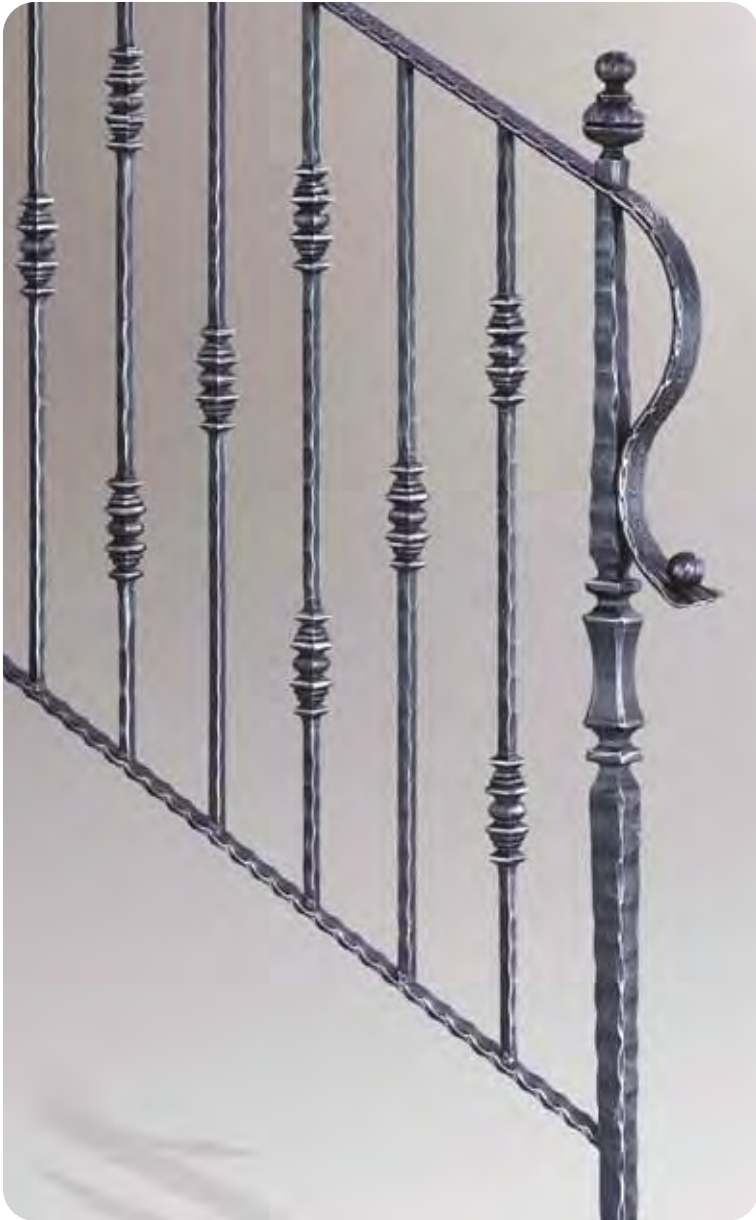
H.3000 mm. Art. 12.037 ≙ 40 X 4 Art. 12.038 ≙ 40 X 8 H.6000 mm. Art. 12.039 ≙ 40 X 4 Art. 12.040 ≙ 40 X 8
