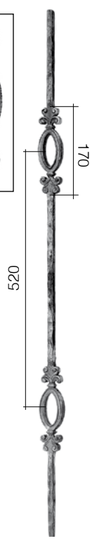
Art. 490/1 Ø 14 x 14 mm H 1000 mm
