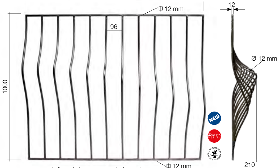
left - sinistro Art. GD294/1 Ø 12 mm 1200 x 1000 mm right - destro Art. GD294/1/S Ø 12 mm 1200 x 1000 mm
