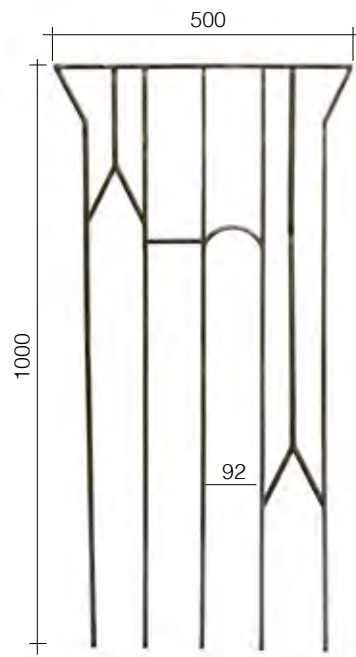
Art. GD295/2 □ 14 x 8 mm 500 x 1000 mm
