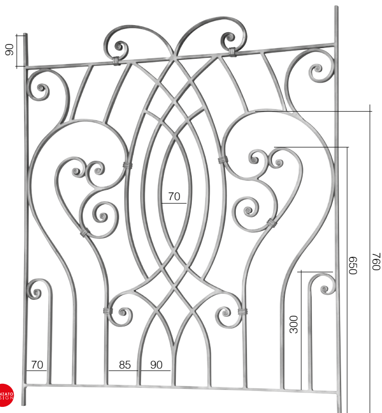
Art. GD235/1 Ø 14 x 8 mm 890 x 1000 mm
