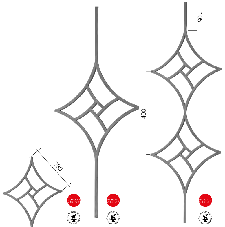
Art. GD211/2 □ 12 mm 395 x 395 mm
