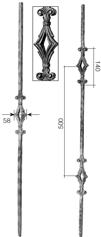
Art. 489/2 Ø 14 x 14 mm H 1000 mm
