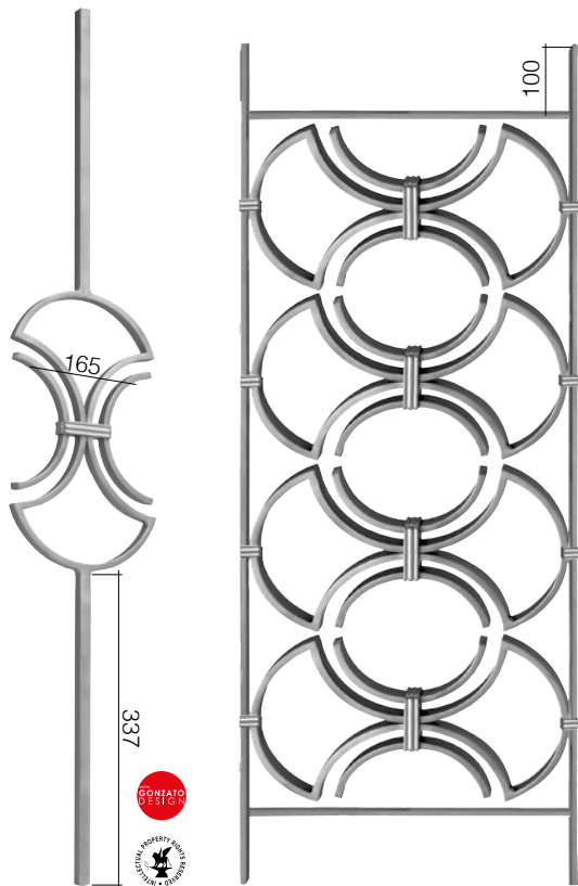
Art. GD187/1 Ø 14 mm 190 x 1000 mm BEST PRICE
