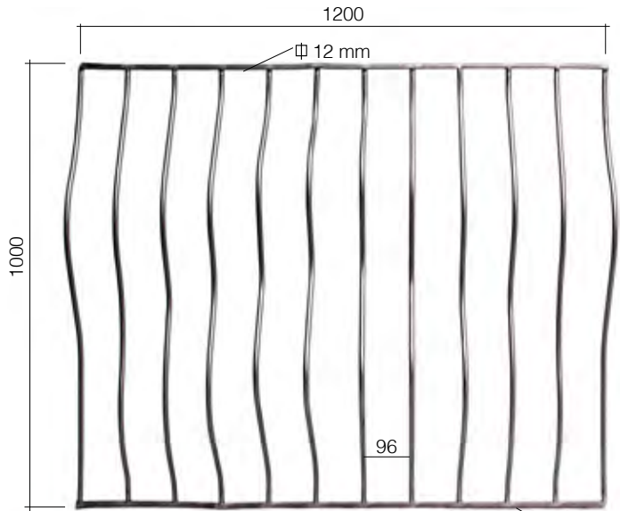
left - sinistro Art. GD294/2 Ø 12 mm 1200 x 1000 mm right - destro Art. GD294/2/S Ø 12 mm 1200 x 1000 mm
