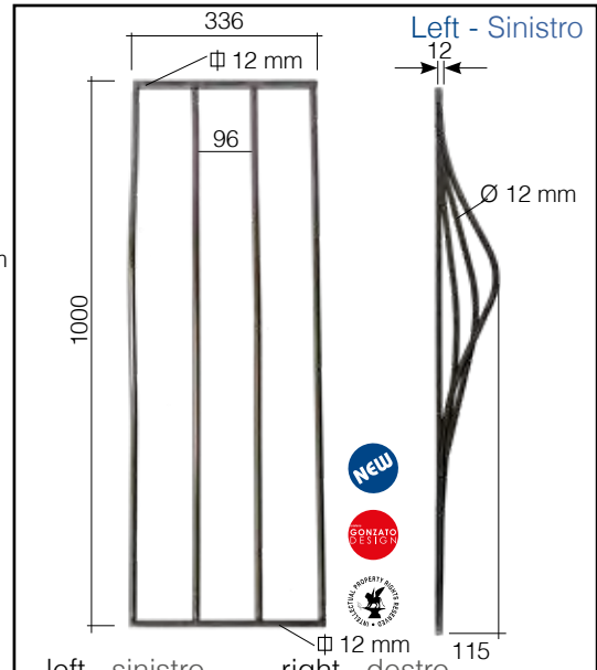
left - sinistro Art. GD294/3 Ø 12 mm 336 x 1000 mm right - destro Art. GD294/3/S Ø 12 mm 336 x 1000 mm
