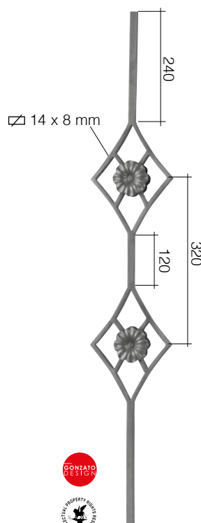
Art. GD18/1 □ 14 x 8 mm 160 x 1000 mm
