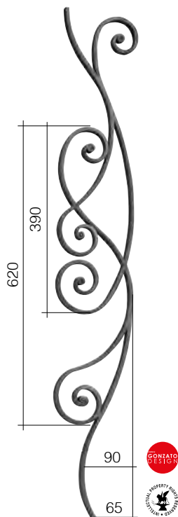
Art. GD158/2 ∅ 14 x 8 mm 160 x 1000 mm
