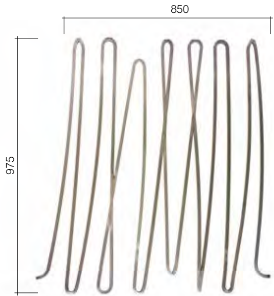
Art. GD300/1 ∅ 12 x 12 mm 850 x 975 mm
