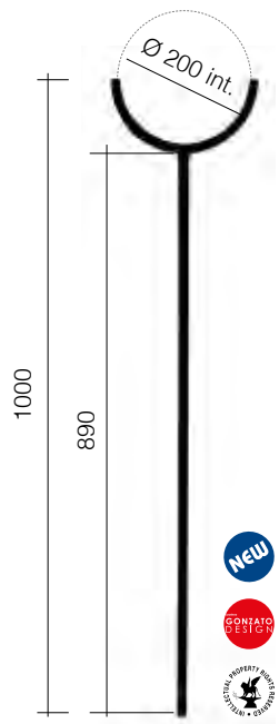
Art. GD296/1 Ø 12 x 12 mm Ø 224 x 1000 mm
