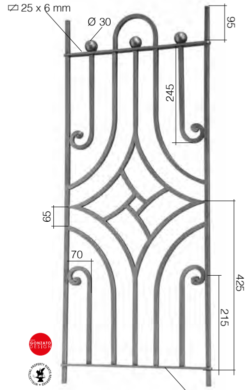
Art. GD212/1 □ 25 x 6 mm □ 12 x 12 mm 420 x 1000 mm
