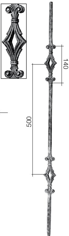
Art. 489/1 Ø 14 x 14 mm H 1000 mm
