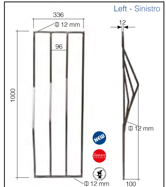
left - sinistro Art. GD293/3 12 x 12 mm 336 x 1000 mm
