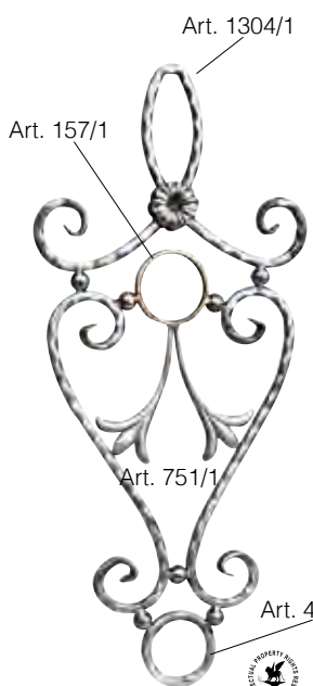
Art. 475/1 hammered - spigolato 12 x 12 mm 380 x 825 mm
