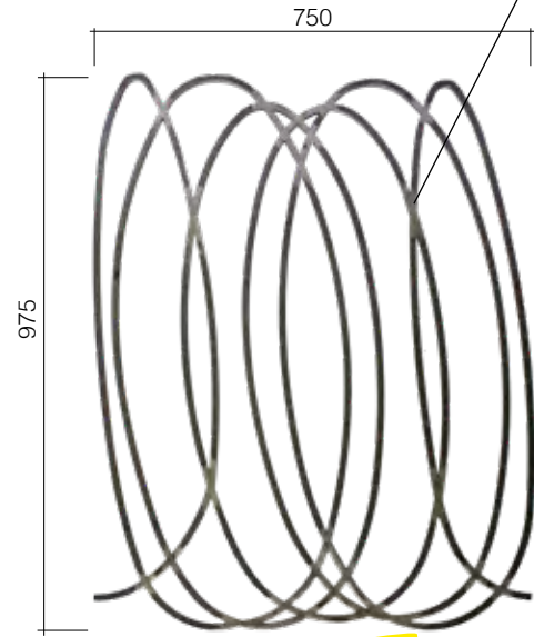
Art. GD300/2 ∅ 12 x 12 mm 750 x 975 mm
