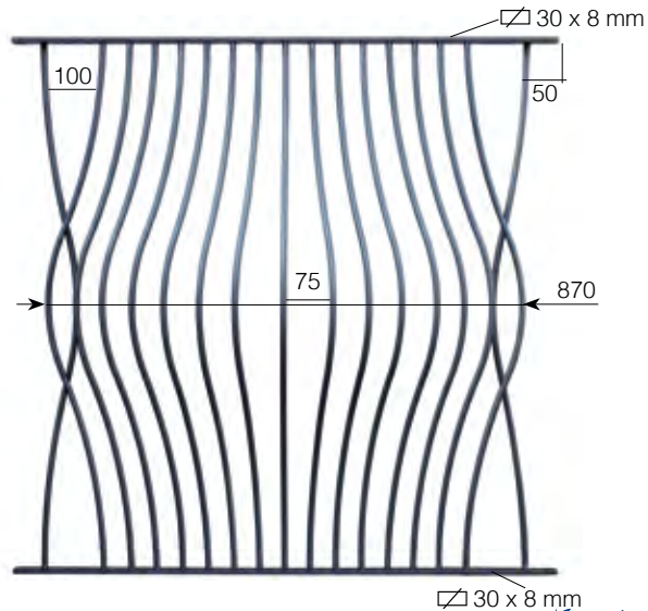
left - sinistro Art. GD294/2 Ø 12 mm 1200 x 1000 mm right - destro Art. GD294/2/S Ø 12 mm 1200 x 1000 mm
